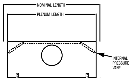
PLENUM SIDE VIEW
