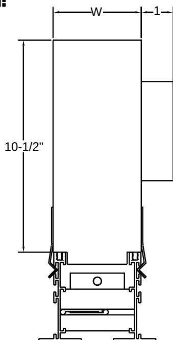
PLENUM (INSTALLED) END VIEW
