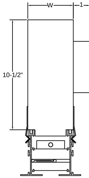
PLENUM (INSTALLED) END VIEW
