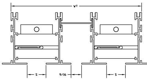
2T SLOT (ACOUSTICAL)
