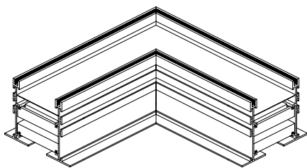
Mitered Corner 90°
