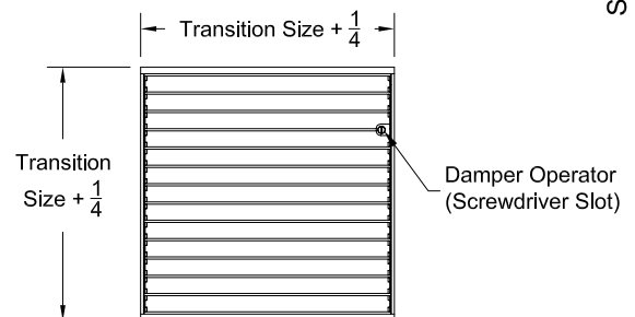
Face View (OBDE-R5 Model)
