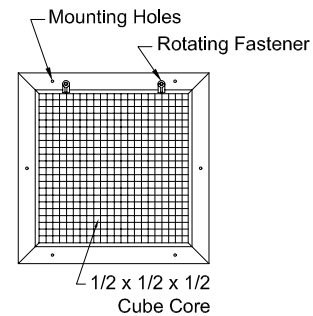
Face view (CC5F-1-GS & CC5F-1-FS)
