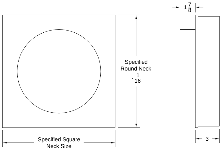
Model: TR-DEEP (Square to Round Deep Transition)
