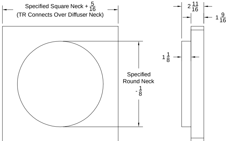
Model: TR (Square to Round Transition)
