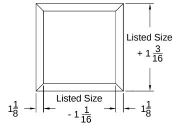
Face View (Models TBPF and STBPF)
