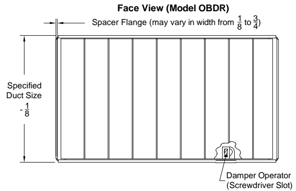
Model: OBDR (Roll Formed Aluminum - Opposed Blade Damper)
