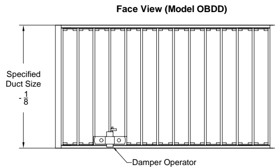
Model: OBDD (Extruded Aluminum - Opposed Blade Duct Damper)
