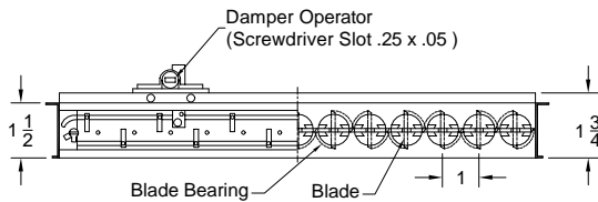
Model: OBDD (Extruded Aluminum - Opposed Blade Duct Damper)
