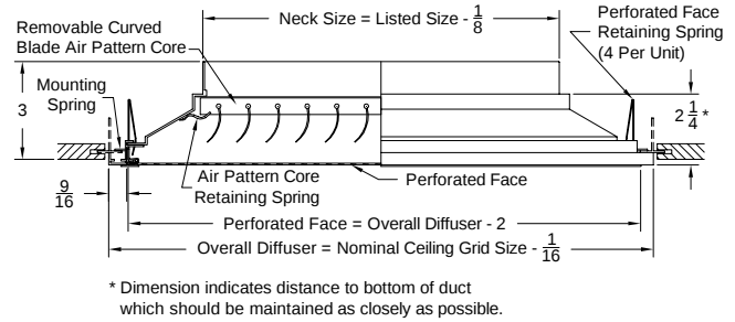
Model: 7000-7 ( Concealed Spline )
