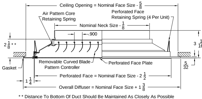
Model: 7000-1 ( Flush Ceiling Mount )
