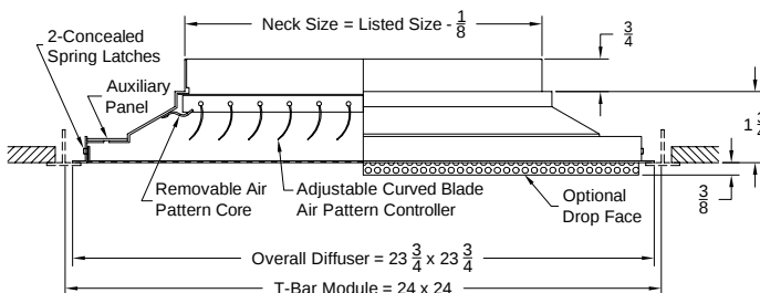
Model: 7000-6 * (Lay in T-Bar 24x24 Grid Size )
