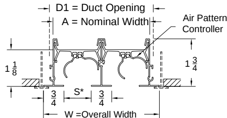
(6600-30-6 Model - End Border)
