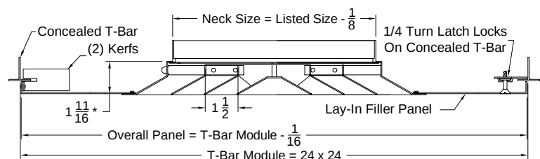
Model: 5000-7 (Concealed Spline)
