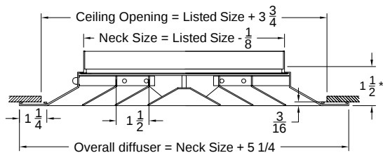
Model: 5000-1 (Flush Surface Mount)
