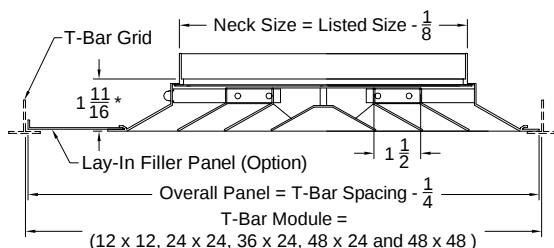
Model: 5000-6 (Lay in T-Bar)
