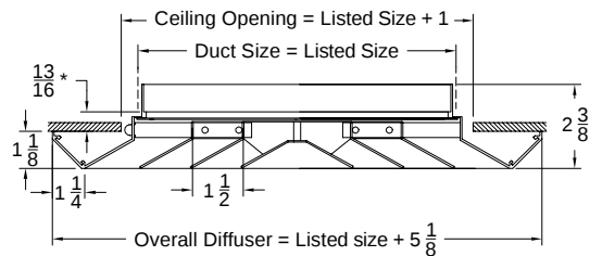
Model: 5000-2 (V-Beveled Drop Surface )
