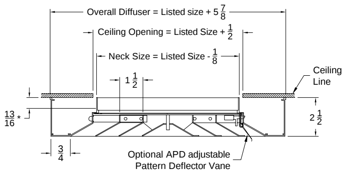
Model: 5000-4 (Deep Drop Surface Mounting)
