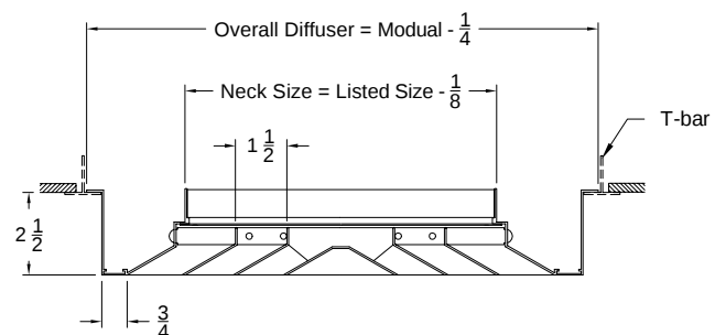
Model: 5000-46 (Lay inT-Bar Deep Drop Surface Mounting)
