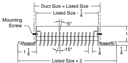
Model: 41C-1 ( Single Deflection Grille ) ( Curved Border )
