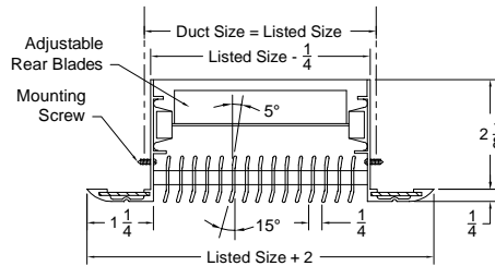
Model: 42C-1 ( Double Deflection Grille ) ( Curved Border )
