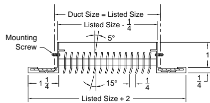
Model: 41F-1 ( Single Deflection Grille ) ( Flat Border )
