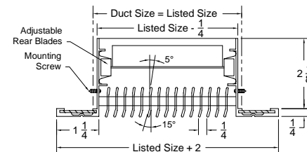
Model: 42F-1 ( Double Deflection Grille ) ( Flat Border )
