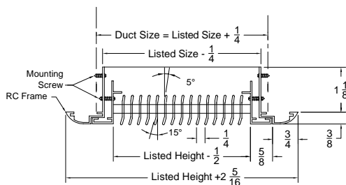
Model: RC41C-1 ( Single Deflection Grille ) ( Curved Border ) ( Removable Inner Frame )
