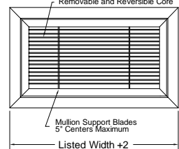
Face view (41C-1,42C-1,41F-1,42F-1) Removable and Reversible Core
