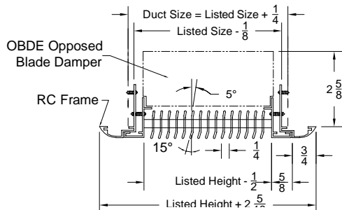
Option: RC41CD-1 ( Single Deflection Register ) ( Curved Border - With OBDE Damper ) ( Removable Inner Frame )
