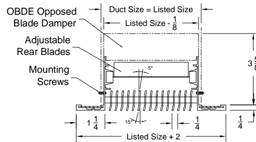
Option: RC42CD-1 ( Double Deflection Register ) ( Curved Border - With OBDE Damper ) ( Removable Inner Frame )
