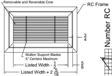
Face view (RC41C-1,RC42C-1) Removable and Reversible Core
