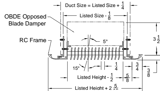
Option: RC42CD-1 ( Double Deflection Register ) ( Curved Border - With OBDE Damper ) ( Removable Inner Frame )
