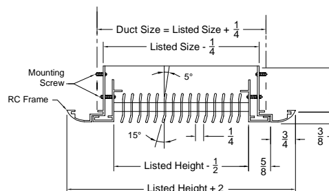
Model: 42F-1 ( Double Deflection Grille ) ( Curved Border ) ( Removable Inner Frame )
