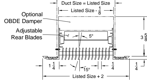
Option: 42FD-1 ( Double Deflection Register ) ( Flat Border - With OBDE Damper )
