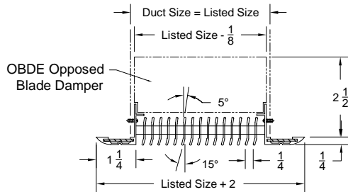
Option: 41FD-1 ( Single Deflection Register ) ( Flat Border - With OBDE Damper )
