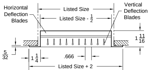
Option: H4004SD-1 ( Double Deflection Register ) ( With OBDR Damper - Horizontal Front Blades )
