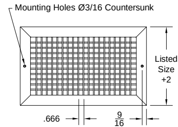
Front View ( Double Deflection ) ( Vertical Front Blades )
