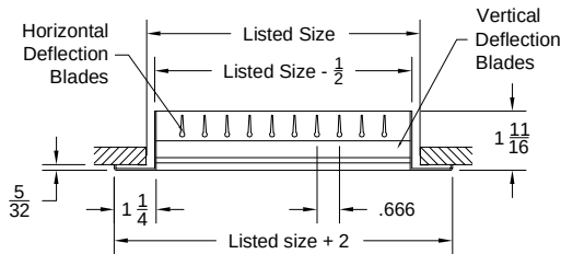
Model: V4004S-1 ( Double Deflection Grille - Vertical Front Blades )
