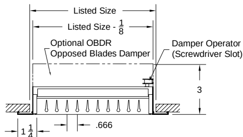
Option: H4004SD-1 ( Double Deflection Register ) ( With OBDR Damper - Horizontal Front Blades )
