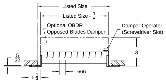
Option: V4004SD-1 (Double Deflection Register) ( With OBDR Damper-Vertical Front Blades )
