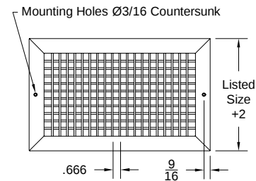
Front View ( Double Deflection ) ( Vertical Front Blades )
