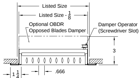
Option: H4004S-AF-1 ( Double Deflection Register ) ( With OBDR Damper - Horizontal Front Blades )
