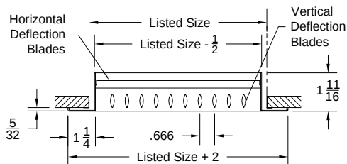
Option: H4004S-AF-1 ( Double Deflection Register ) ( With OBDR Damper - Horizontal Front Blades )
