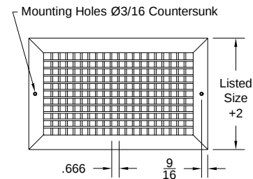
Front View ( Double Deflection ) ( Horizontal Front Blades )
