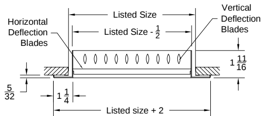
Model: V4004S-AF-1 ( Double Deflection Grille - Vertical Front Blades )
