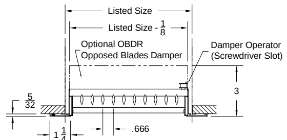
Option: V4004S-AF-1 (Double Deflection Register) ( With OBDR Damper-Vertical Front Blades )
