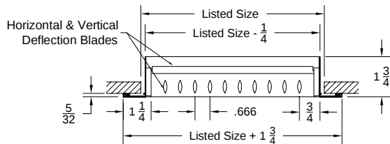
Model: H4004-AF-1 (Double Deflection Grille) (Horizontal Front Blades)
