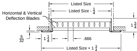
Model: V4004-AF-1 (Double Deflection Grille) (Vertical Front Blades)
