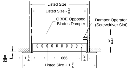
Model: V4004-AF-1 (Double Deflection Register) (OBDE Damper-Vertical Front Blades)
