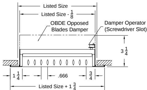
Model: H4004-AF-1 (Double Deflection Register) (OBDE Damper-Horizontal Front Blades)
