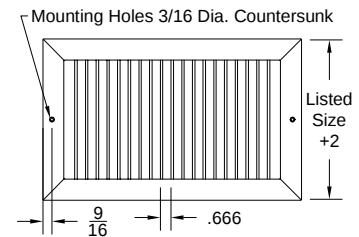
Front View ( Vertical Blades )
