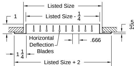
Option: H4002SD-1 (Single Deflection Register) (With OBDR Damper-Horizontal Blades)
