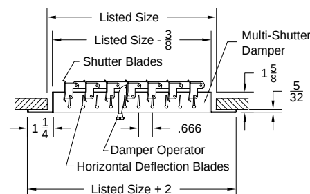
Option: H4002SM-1 (Single Deflection Register) (Multi Shuter Damper-Horizontal Deflection Blades)
