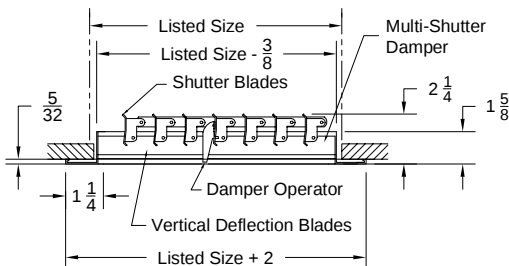
Option: V4002SM-1 (Single Deflection Register) (Multi Shuter Damper-Vertical Deflection Blades)
