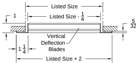
Option: V4002SD-1 (Single Deflection Register) ( With OBDR Damper-Vertical Blades )
