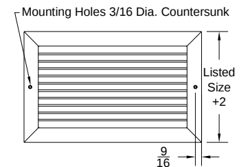
Option: H4002SM-1 (Single Deflection Register) (Multi Shuter Damper-Horizontal Deflection Blades)
