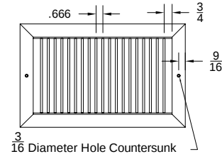
Face View (Vertical Blades)
