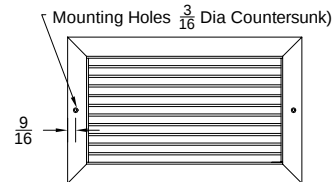
Face View (Horizontal Blades)
