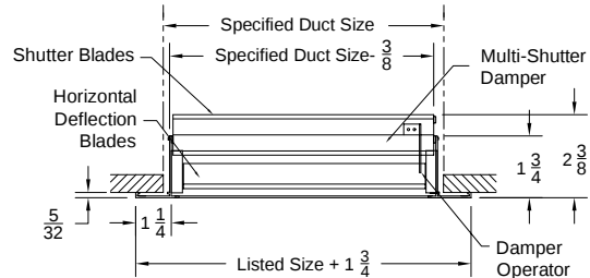
Model: H4002S-AF-1 ( Single Deflection Register ) ( With OBDE Damper-Horizontal Blades )
