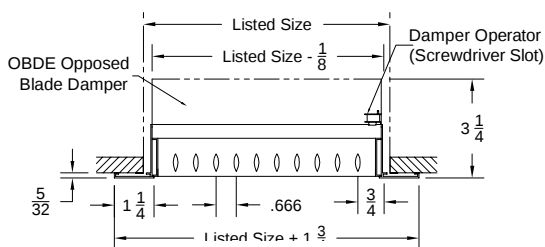
Model: V4002S-AF-1 ( Single Deflection Register ) ( With OBDE Damper-Vertical Blades )
