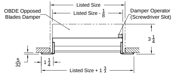
Model: H4002S-AF-1 ( Single Deflection Register ) ( With OBDE Damper-Horizontal Blades )
