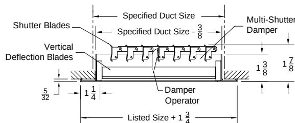
Model: V4002M-1 (Single Deflection Register) (Multi Shutter Damper-Vertical Blades)
