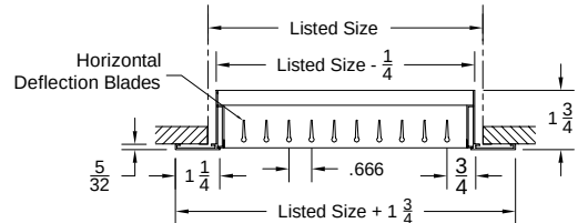
Model: V4002M-1 (Single Deflection Register) (Multi Shutter Damper-Vertical Blades)
