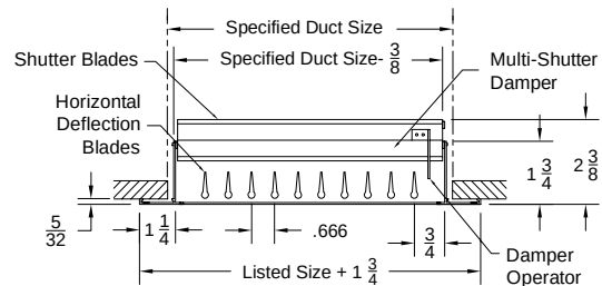
Model: H4002D-1 ( Single Deflection Register ) ( With OBDE Damper-Horizontal Blades )
