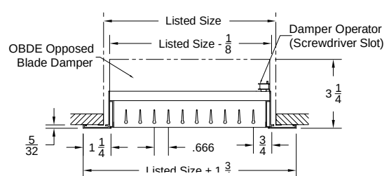
Model: H4002D-1 ( Single Deflection Register ) ( With OBDE Damper-Horizontal Blades )
