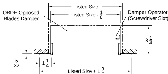
Model: V4002D-1 ( Single Deflection Register ) ( With OBDE Damper-Vertical Blades )
