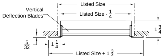
Model: V4002-1 ( Single Deflection Grille - Vertical Blades )
