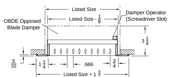
Model: H4002-AF-1 ( Single Deflection Register ) ( With OBDE Damper-Horizontal Blades )
