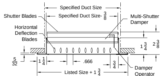
Model: H4002-AF-1 ( Single Deflection Register ) ( With OBDE Damper-Horizontal Blades )
