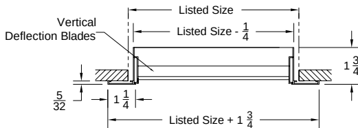
Model: V4002-AF-1 ( Single Deflection Grille - Vertical Blades )
