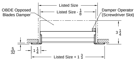
Model: V4002-AF-1 ( Single Deflection Register ) ( With OBDE Damper-Vertical Blades )
