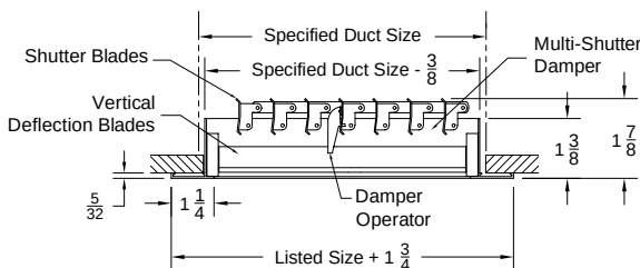
Model: V4002M-AF-1 (Single Deflection Register) (Multi Shutter Damper-Vertical Blades)
