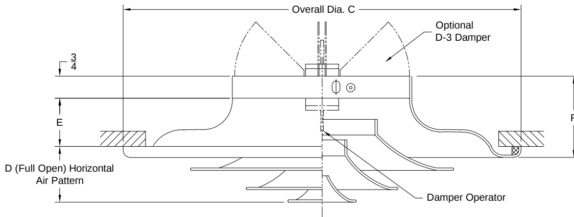
Model: 3000-1D ( Flush Cone with D3 Damper )
