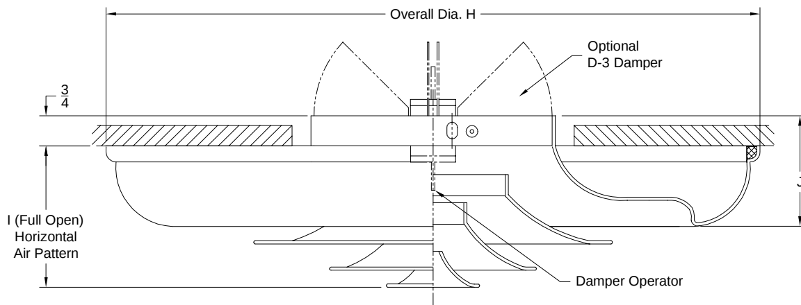
Model 3000-2D ( Drop Cone with D3 Damper )
