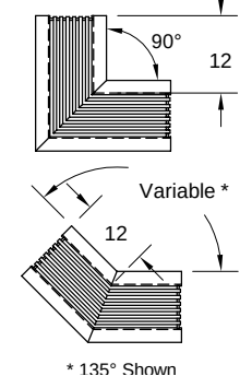
Option: Mitered Corner
