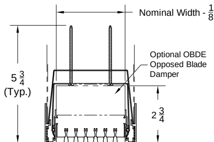
Option: 2100 HWD, 2115 HWD, 2130 HWD (With Damper)
