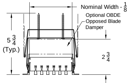
Option: 2100 HD, 2115 HD, 2130 HD (With Damper)
