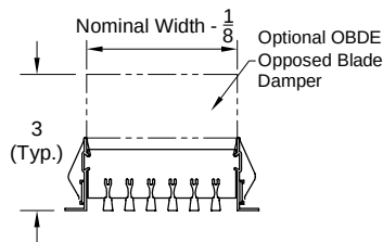
Option: 2100D, 2115D, 2130D (With Damper)
