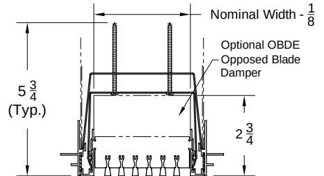
Option: 2100 HPD, 2115 HPD, 2130 HPD (With Damper)
