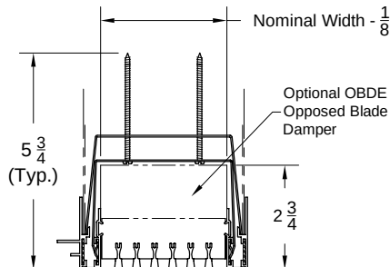
Option: 2100 HCD, 2115 HCD, 2130 HCD (With Damper)
