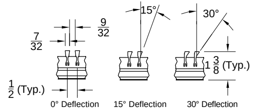
Option: 0°, 15° or 30° Deflection
