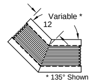
Option: Mitered Corner Sections
