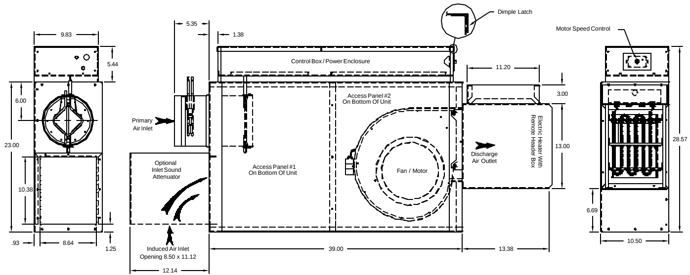
TOP VIEW
