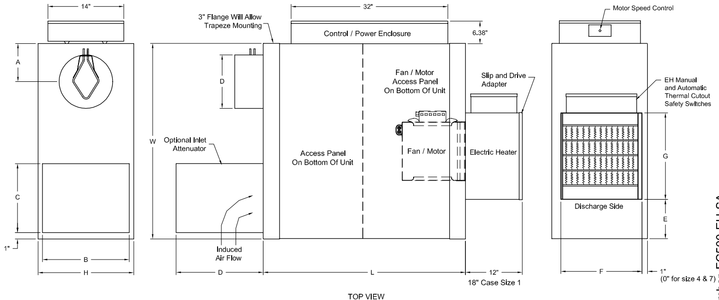
TOP VIEW
