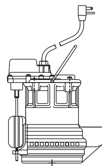
247 VMF-Series (U.S. Patent #5324171) VMF switch, magnetically operated vertical float – operates in a 10" diameter sump.
