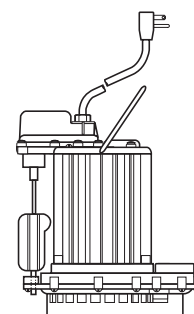
Model 237 VMF VMF Switch, mag- netically operated for smaller pits down to 10" diameter (U.S. Patent # 5324171)
