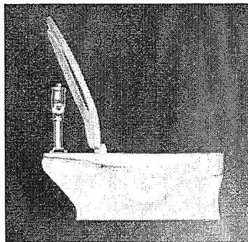
Self-Sustaining Check Hinge - External self-sustaining check hinge holds seat in any raised position up to 11 degrees beyond vertical
