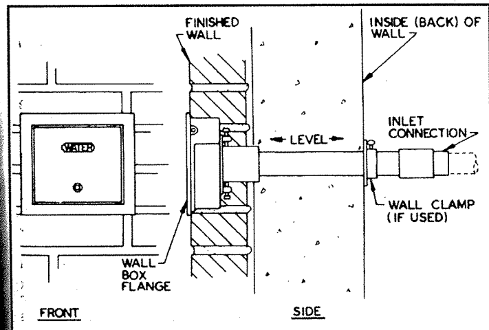
HYDRASAN I 71000 INSTALLATION FIGURE 1
