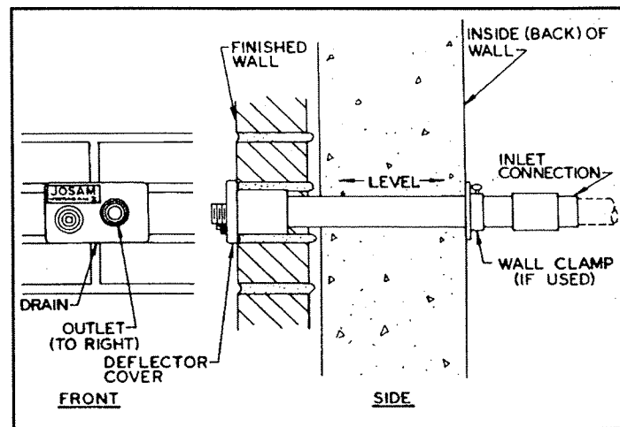
HYDRASAN I 71050 INSTALLATION FIGURE 2
