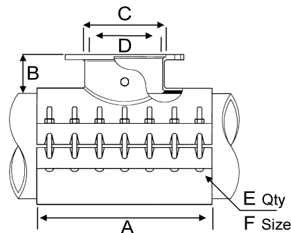
JCM 432 & 462 STAINLESS STEEL TAPPING SLEEVE DIMENSIONS
