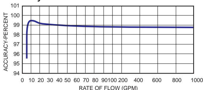
Accuracy Curve
