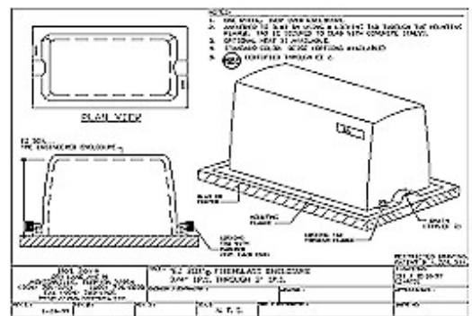
Ez Box fiberglass enclosure
