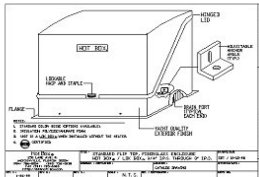
Standard Flip-top fiberglass enclosure
