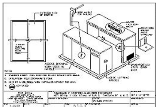
Standard 2-pc Aluminum Enclosure
