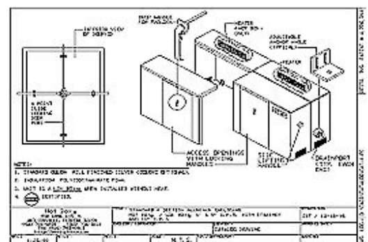
Standard 4-pc Aluminum Enclosure
