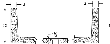
SECTION THRU THRESHOLD
