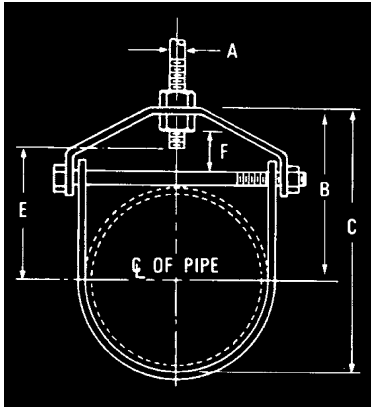
FIG. 11 STANDARD CLEVIS HANGER, DOMESTIC FIG. 11GI STANDARD CLEVIS HANGER, ELECTRO-GALVANIZED
