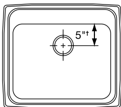
±4-1/2" for LRAD(Q)1522 Off-Centered Rear
