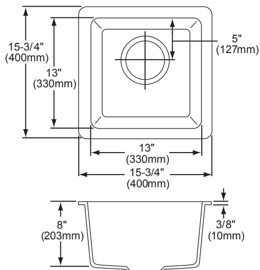
Cross Profile of Installation
