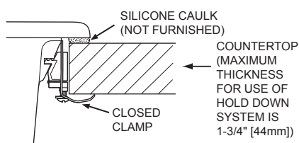
Cross Profile of Installation A
