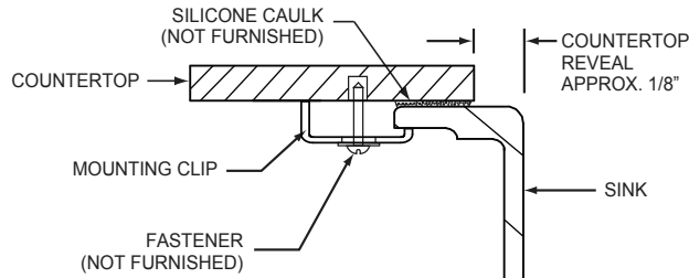
Cross Profile of Installation B
