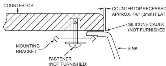
Cross Profile of Installation
