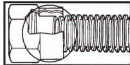
Dormont No-Neck™ Construction
