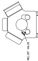
RELIEF VALVE LOCATED ON THE COMPRESSOR FIELD CONNECTION WITH A 3/8" SAE FLARE FOR FIELD CONNECTION SCALE 1:8
