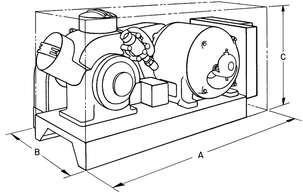
COMPRESSOR UNIT, BELT DRIVE (BD)
