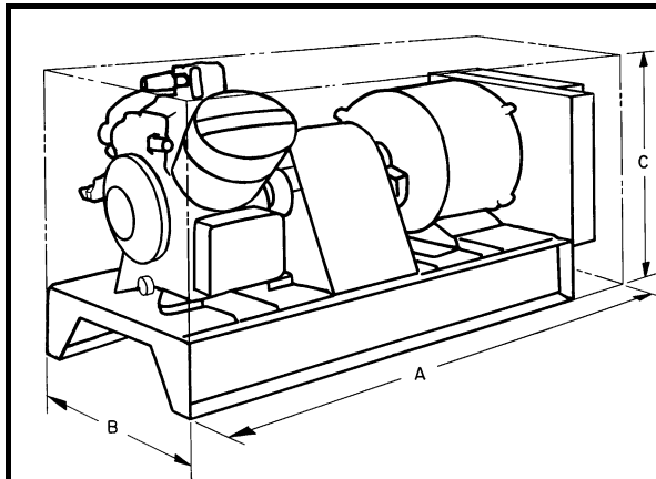
COMPRESSOR UNIT, DIRECT DRIVE (DD)
