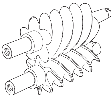
TWIN-SCREW COMPRESSOR DESIGN
