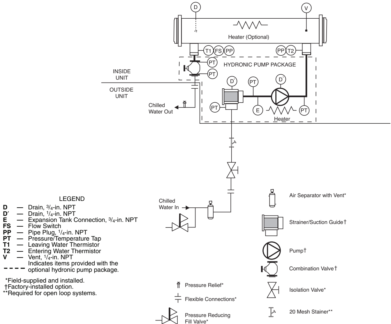
TYPICAL PIPING DIAGRAM FOR 30RB UNITS WITH HYDRONIC PACKAGE — SINGLE PUMP
