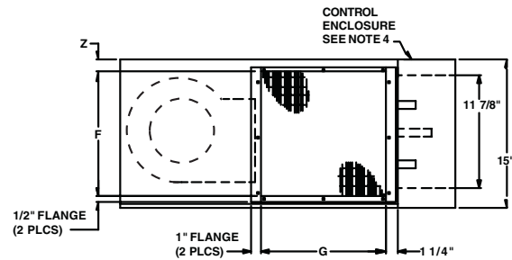
DISCHARGE VIEW
