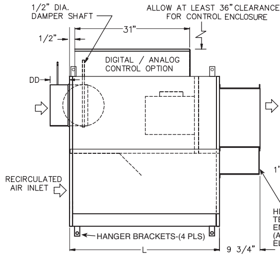
PLAN VIEW — LEFT HAND UNIT SHOWN RIGHT HAND AVAILABLE (CONTROLS NOT SHOWN)
