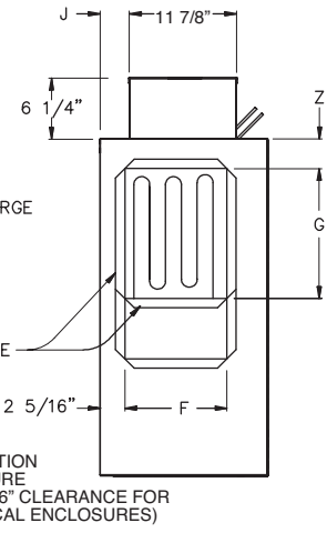
DISCHARGE VIEW
