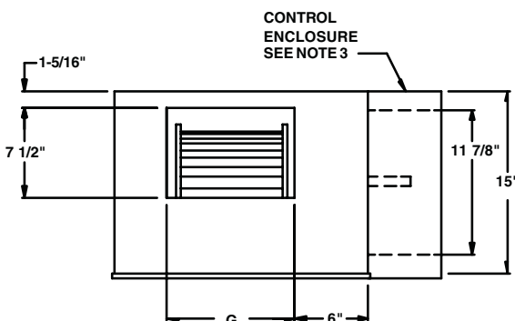
DISCHARGE VIEW
