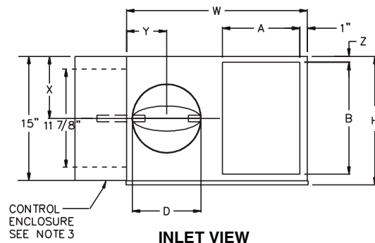
INLET VIEW
