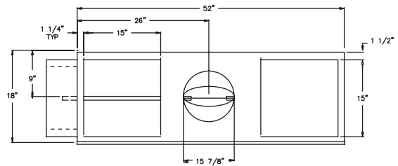
INLET VIEW
