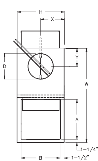
INLET VIEW
