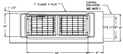
DISCHARGE VIEW
