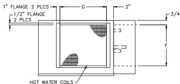
DISCHARGE VIEW
