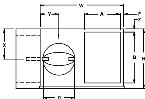
INLET VIEW
