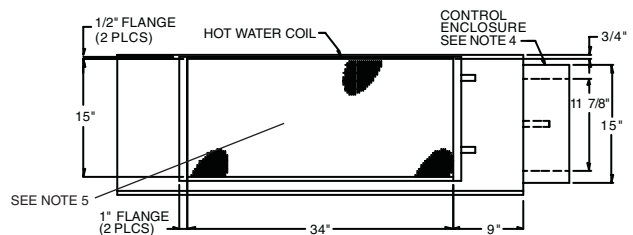
DISCHARGE VIEW
