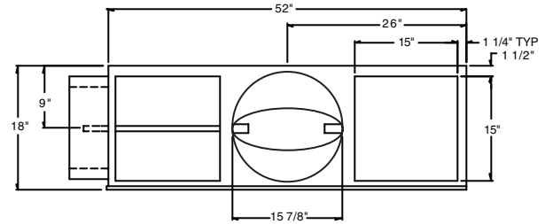
INLET VIEW
