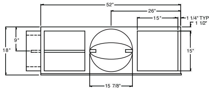
INLET VIEW
