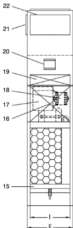
FRONT VIEW
