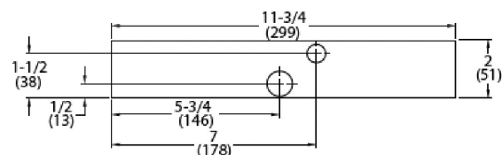
DRAIN OUTLET
