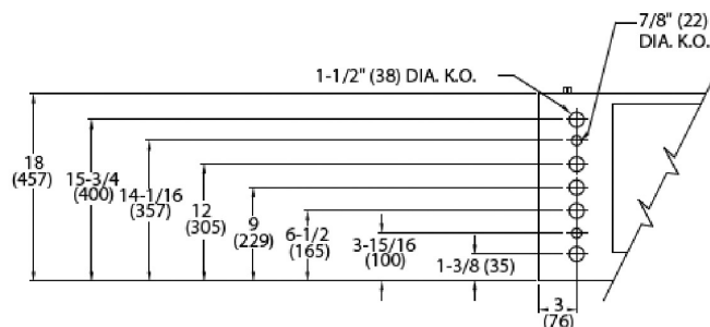
PARTIAL REAR VIEW (TYP. BOTH SIDES)
