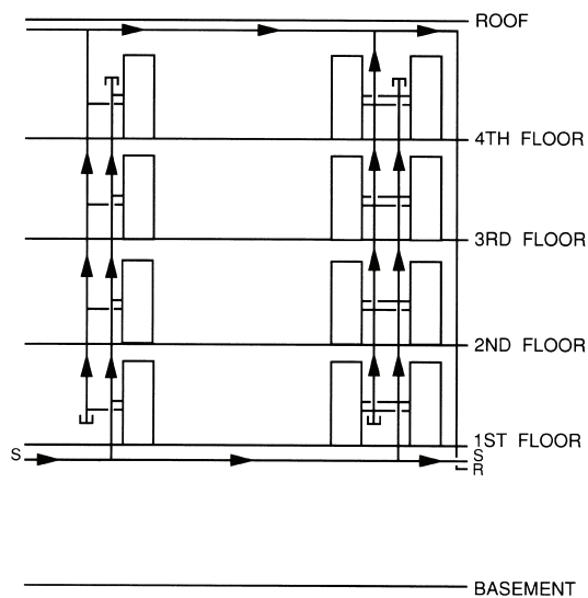
SYSTEM 3 — COMMON REVERSE RETURN
