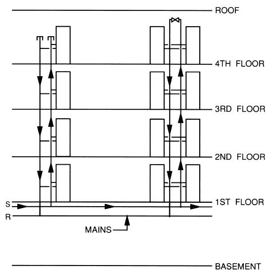
SYSTEM 1 — DIRECT RETURN
