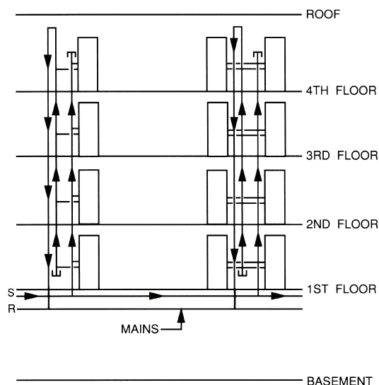
SYSTEM 2 — REVERSE RETURN
