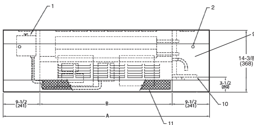
FRONT VIEW
