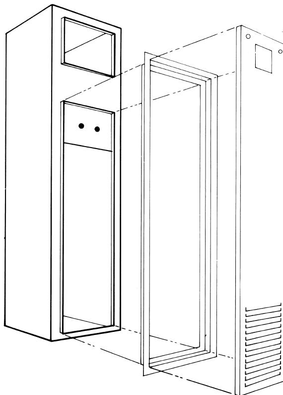
LONG FRAME — FLUSH MOUNTED GRILLE
