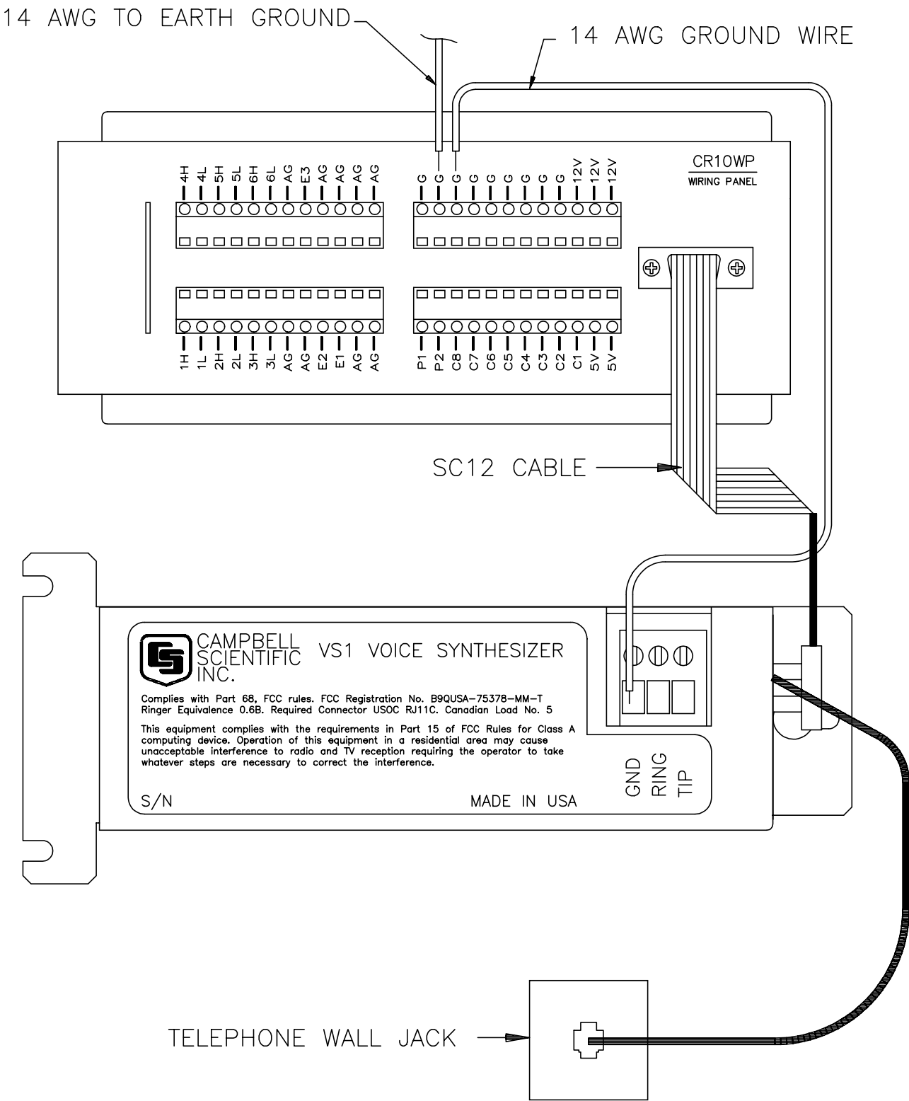
FIGURE 3-2. Standard Telephone Jack Connection
