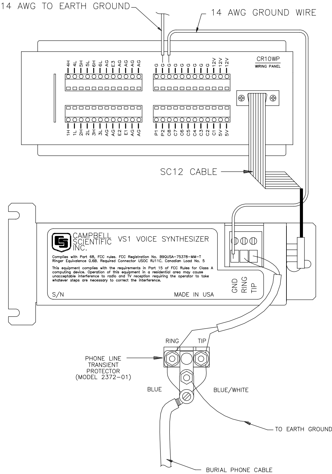
FIGURE 3-3. Remote Site Connection
