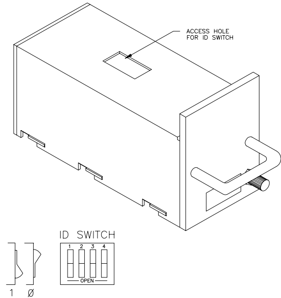
FIGURE 3-1. Address Switch on SDM1502
