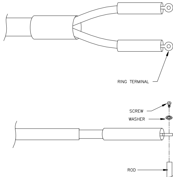
FIGURE 3-4. SDM Wiring
