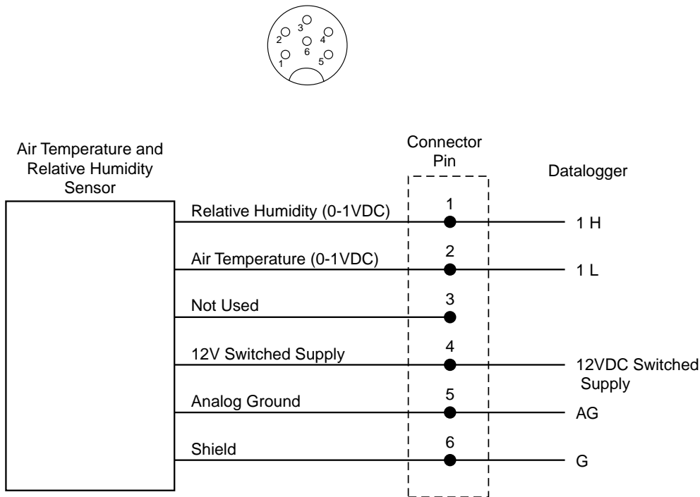
FIGURE 4.10-1. Schematic of CS500-LC RH and Temperature Probe and Connector #1
