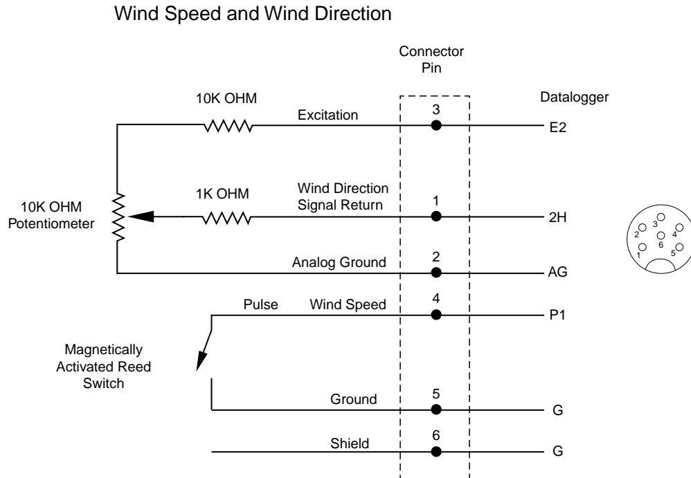
FIGURE 4.10-2. Schematic of 034A-LC Wind Speed and Direction Probe and Connector #2
