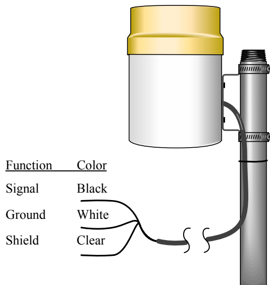
FIGURE 1. TE525 Tipping Bucket Rain Gage
