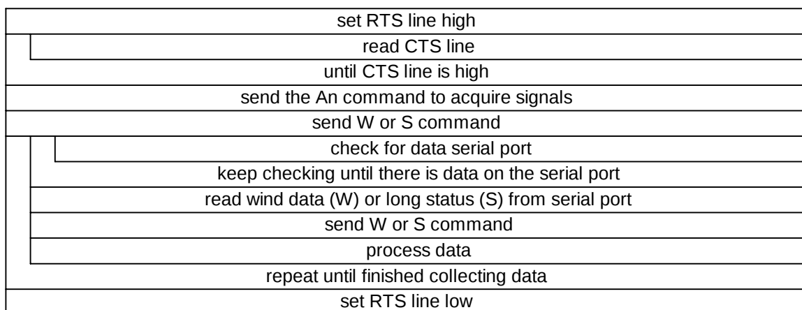
FIGURE B-2. CSAT3 as the Trigger Source.
