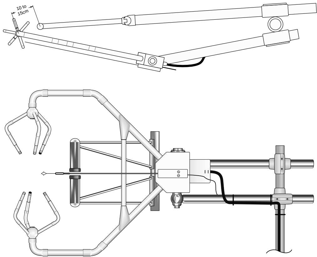
FIGURE 4-2. CSAT3 Sonic Anemometer, KH20 Krypton Hygrometer, and FW05 Fine Wire Thermocouple.
