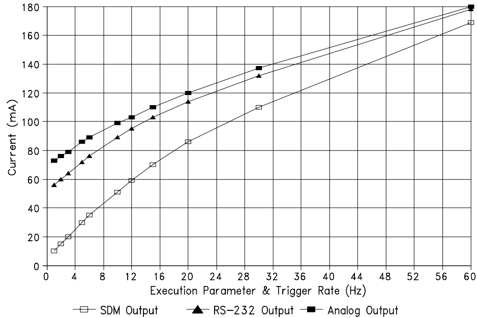
FIGURE 8-1. Typical Average CSAT3 Power Requirements at +12 VDC
