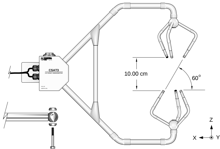
FIGURE 4-1. CSAT3 Coordinate System and Mounting Hardware
