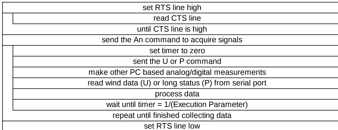
FIGURE B-1. PC as the Trigger Source.
