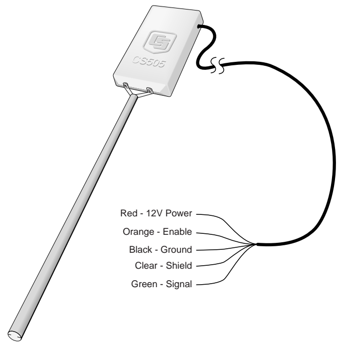
FIGURE 3. CS505 Wire Color and Function
