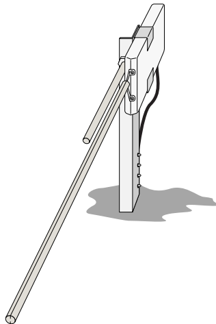
FIGURE 2. CS505 Installation Options Over Forest Floor, 30cm Over Duff Layer
