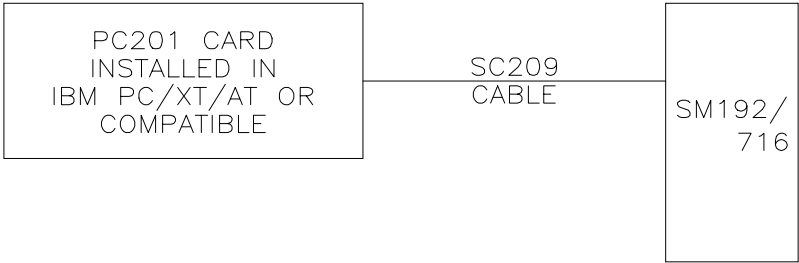
5.1-2 Storage Module Connected to PC201 Card
