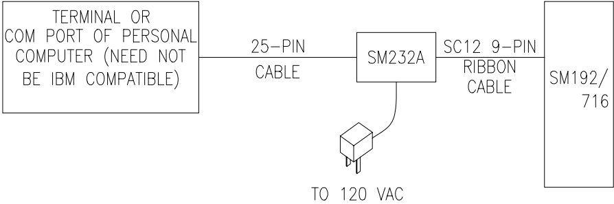
5.1-4 Storage Module Connected With SM232A
