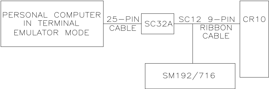
5.1-3 Communication Via the CR10
